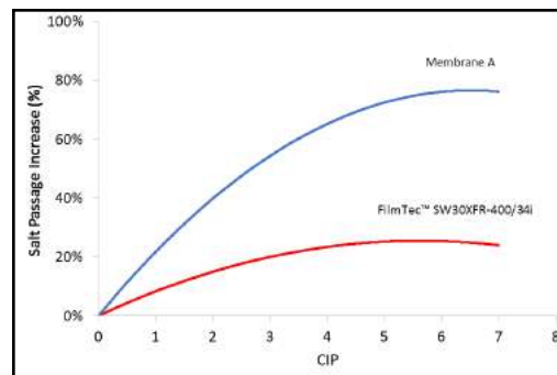
Figure 1: Salt Passage Increase versus number of CIP for SW30XFR-400/34i and Membrane A
